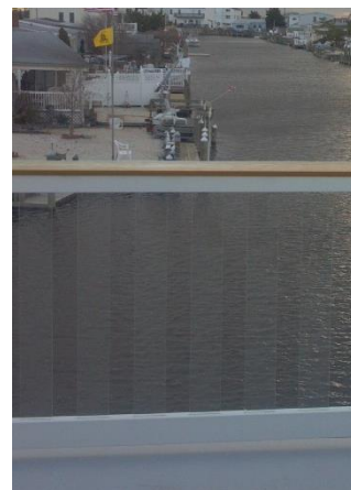
2" x 3.5" Top & Bottom Rail with 4" wide Glass Balusters
